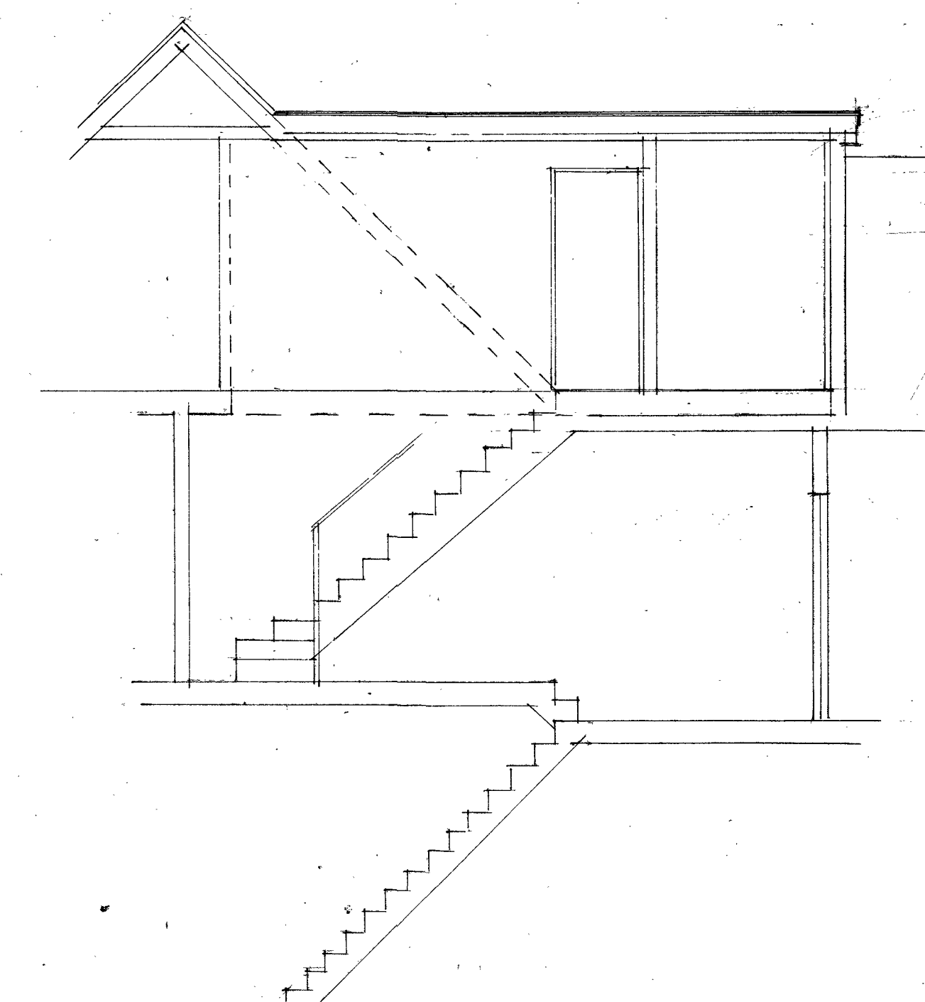
TEST SECTION FOR STAIR HEADHEIGHT. 1:50.
