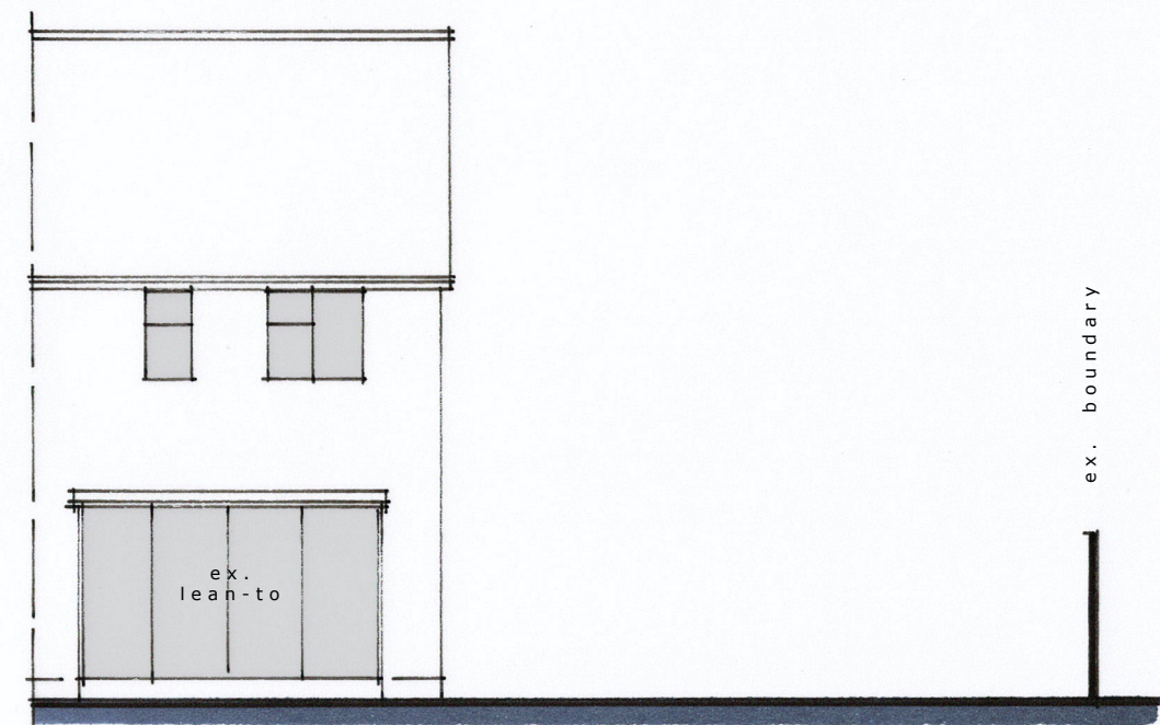
REAR (s)
