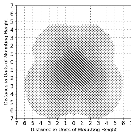
Isoillumiance Plot
