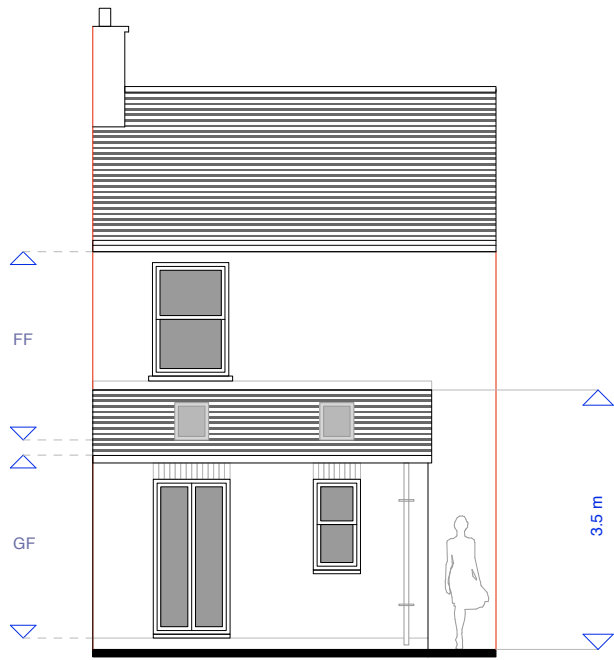
Proposed Rear Elevation at 1:100 scale WEST
