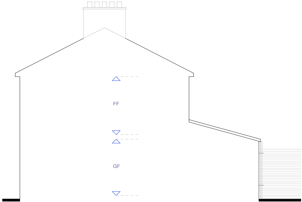
Proposed Side Elevation at 1:100 scale NORTH
