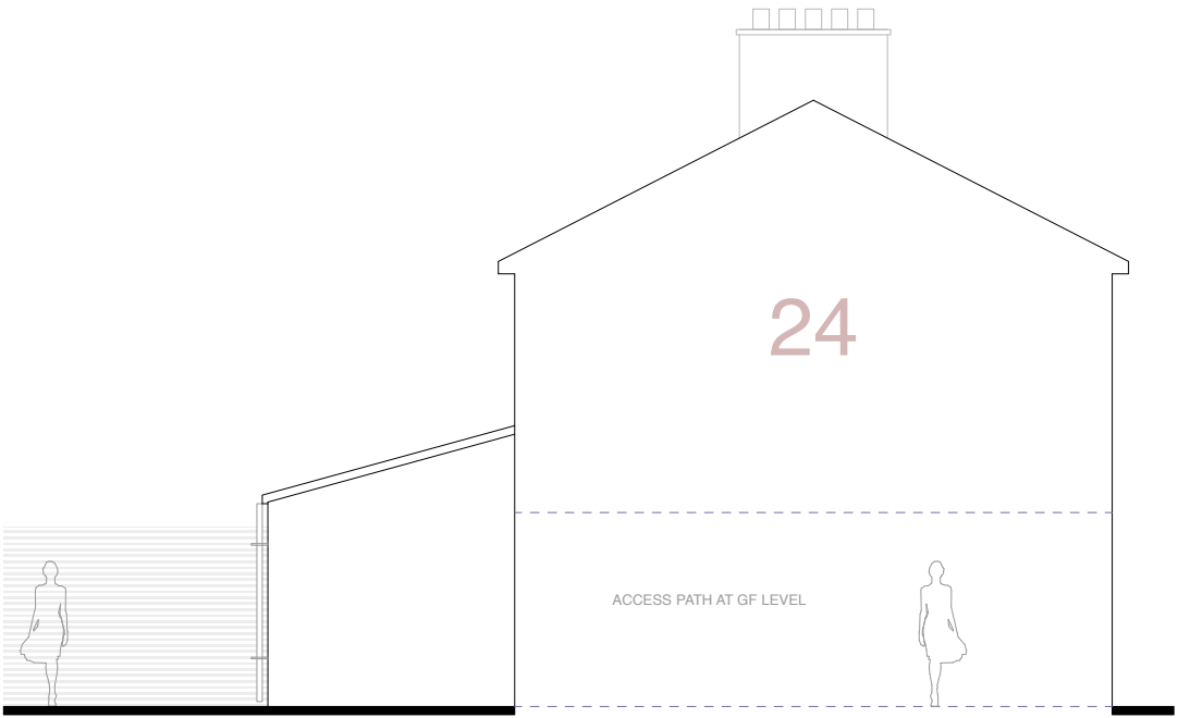
Proposed Side Elevation at 1:100 scale SOUTH
