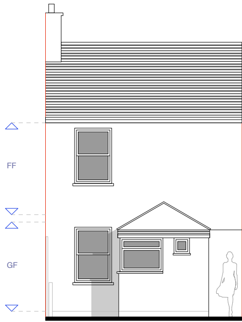
Existing Rear Elevation at 1:100 scale WEST
