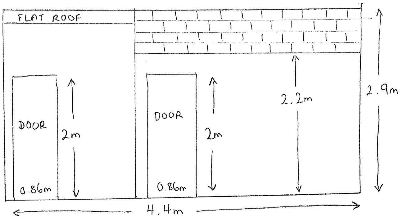
WEST-FACING CURRENT ELEVATION
