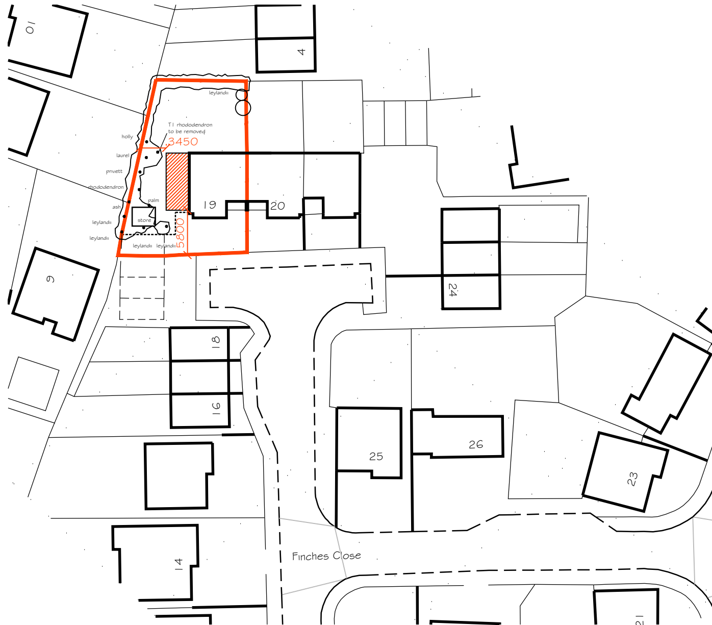
Block Plan
