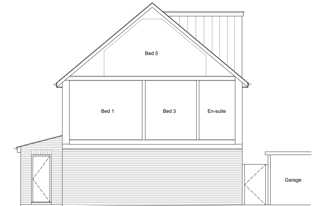
East Sectional Elevation
