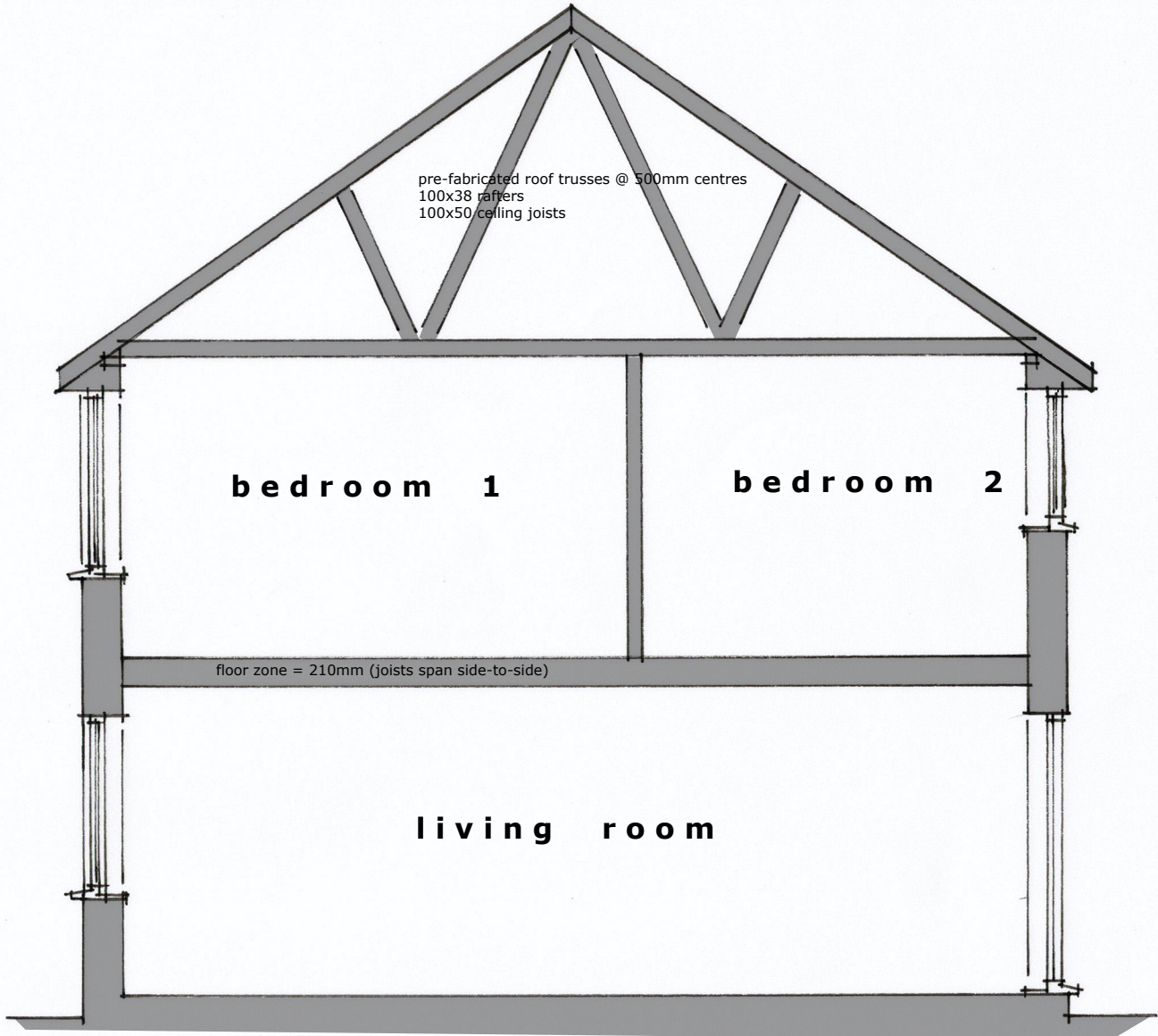
SECTION 1:50
