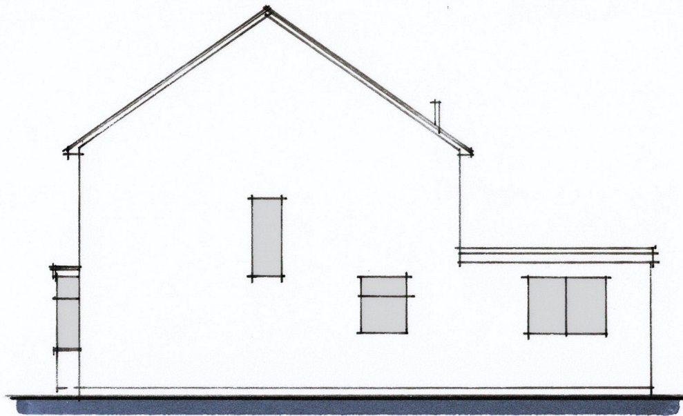
SIDE (s) ELEVATION 1:100 @ A3
