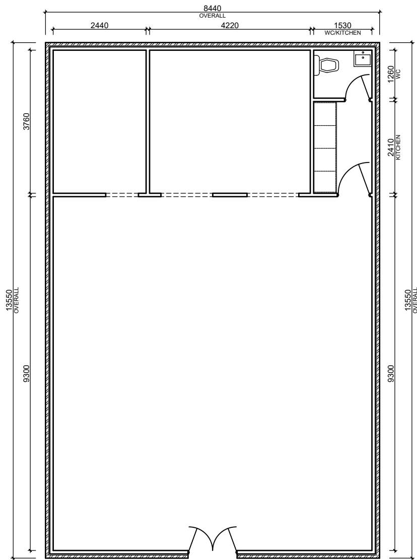
EXISTING FLOOR PLAN Scale: 1/100
