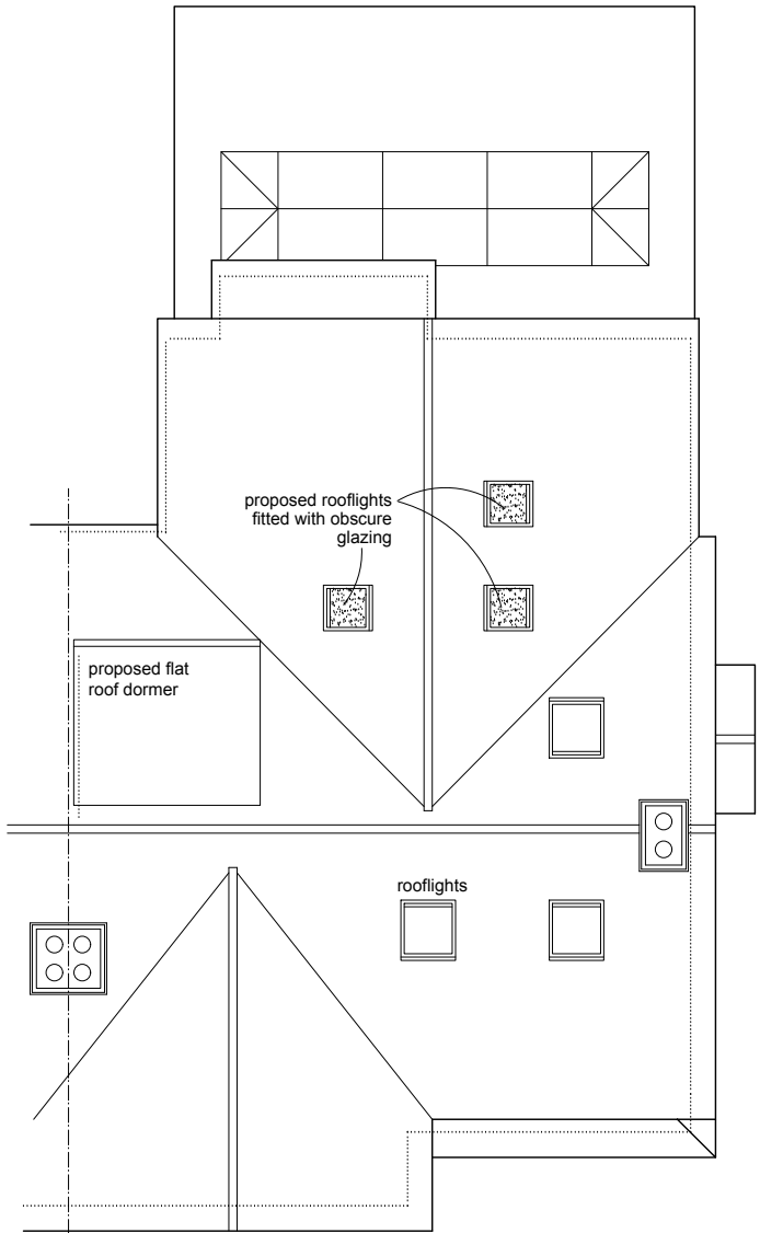
Roof Plan
