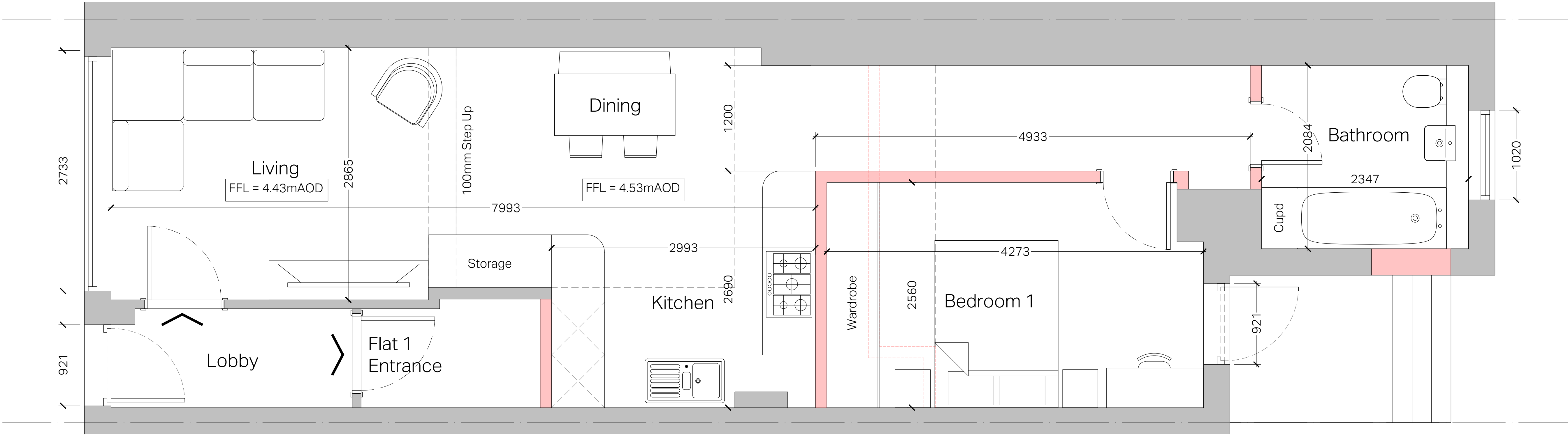
Ground Floor Plan - Proposed (49.2m 2 Plot Total) (NDSS 1 Bed, 1 Person = 39m 2 )
