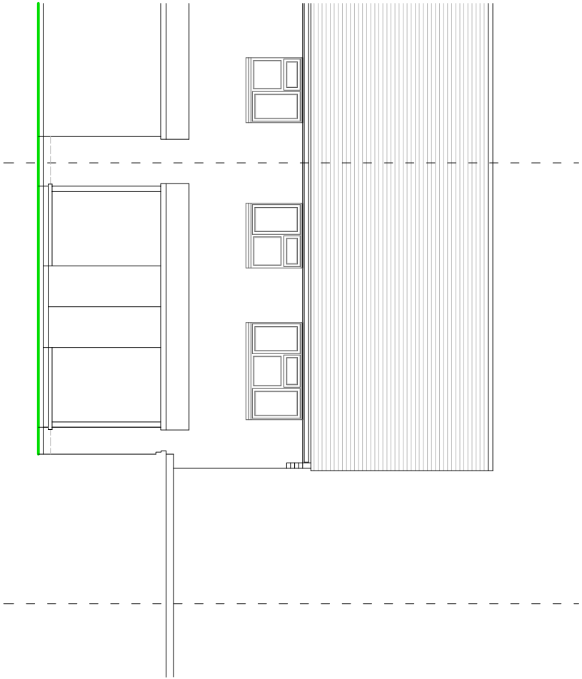
REAR ELEVATION
