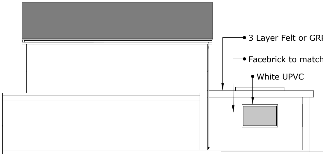
A :: Proposed West Elevation 04 scale: 1:100
