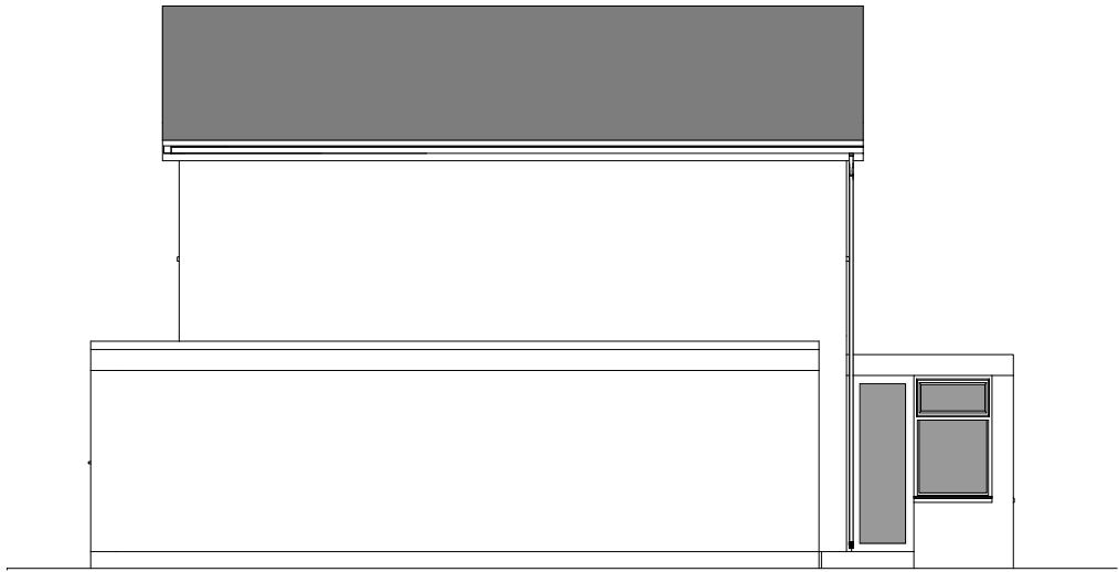
A :: Existing west Elevation 02 scale: 1:100
