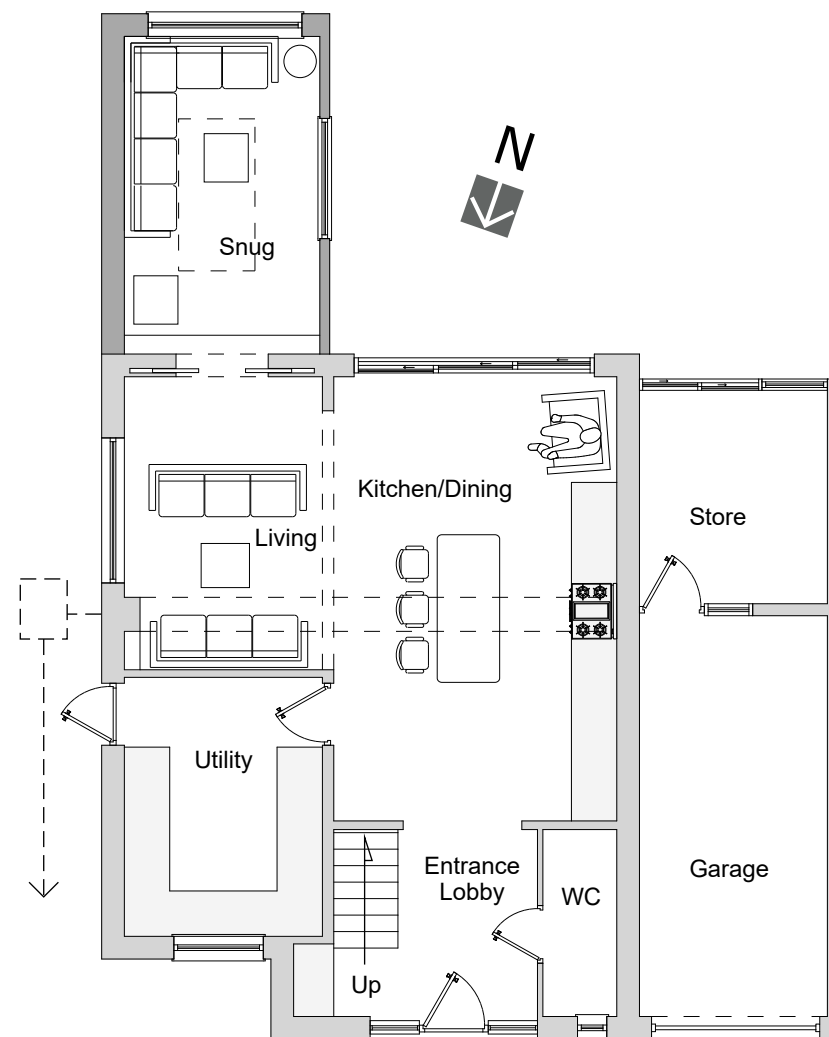
A :: Proposed Ground Floor Plan 03 scale: 1:100
