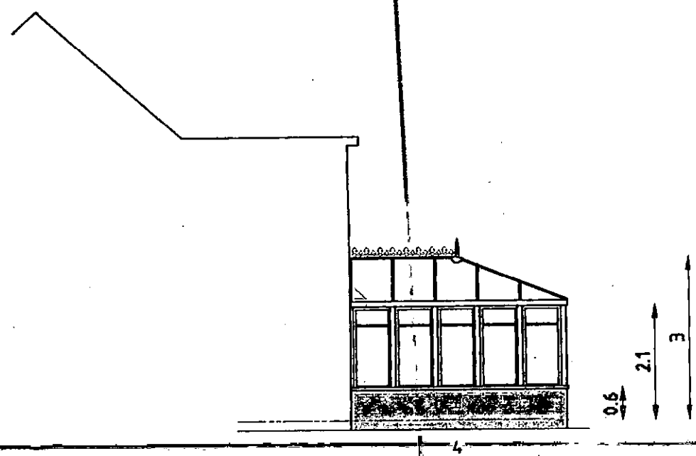
South Elevation
