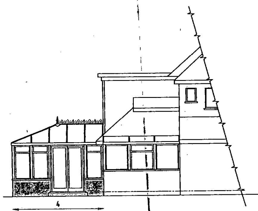
North Elevation
