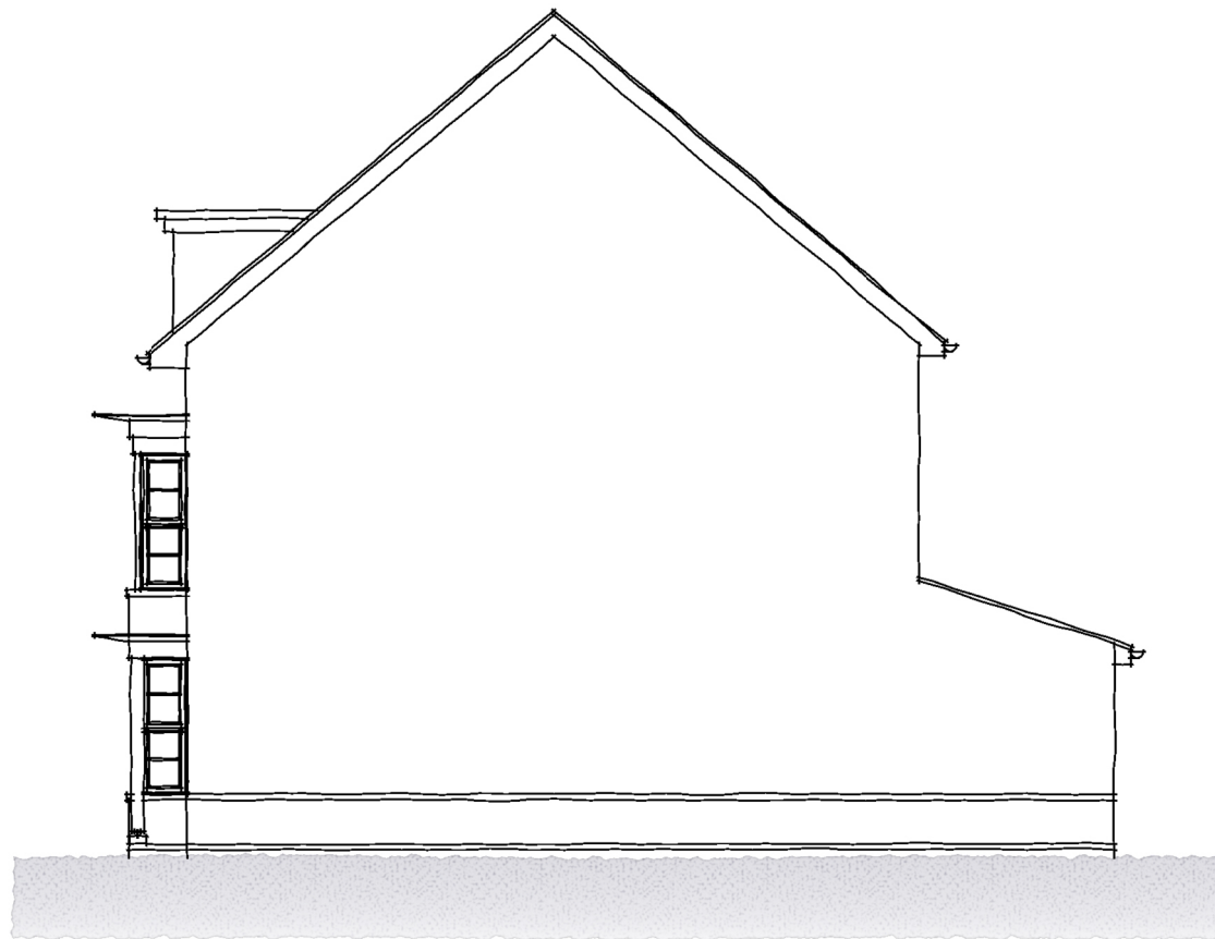
SIDE ELEVATION
