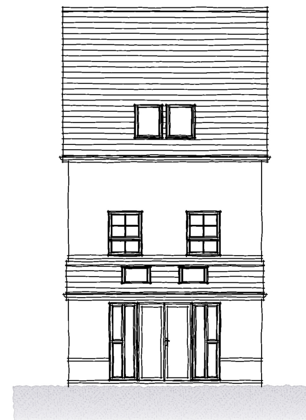
REAR ELEVATION
