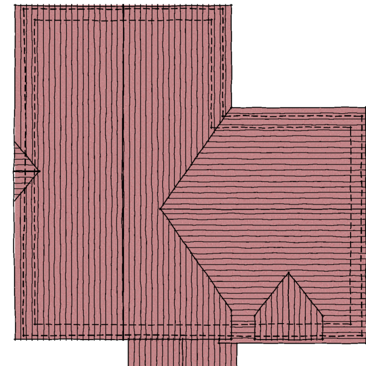
ROOF PLAN
