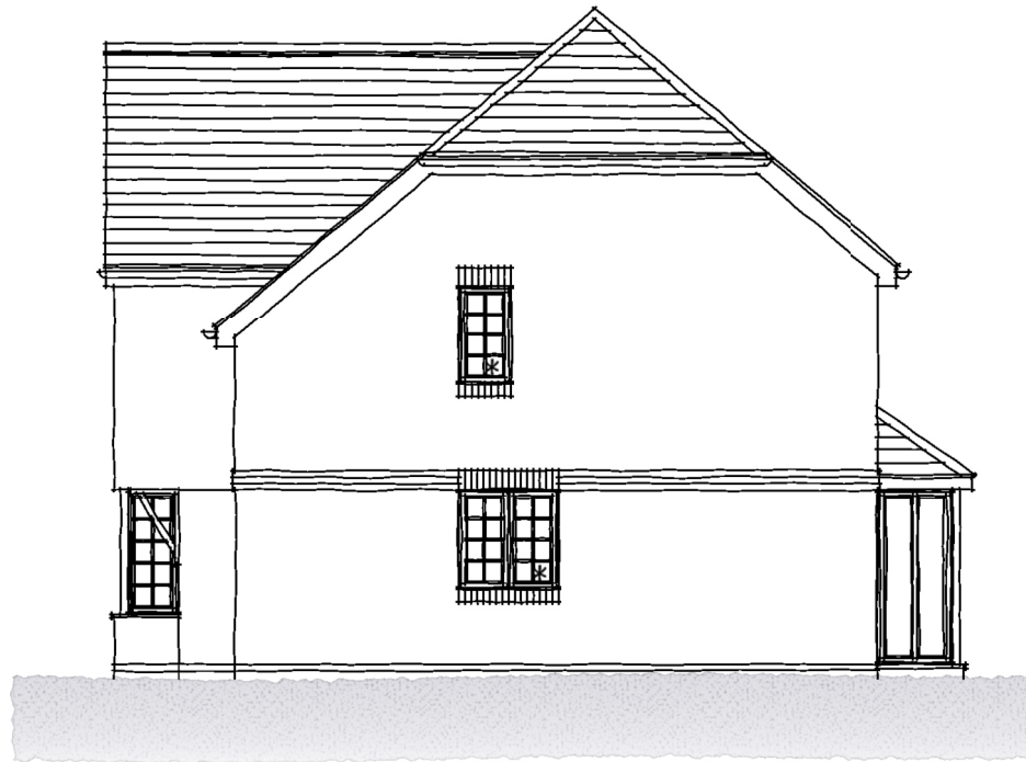
SIDE ELEVATION * WINDOWS TO PLOTS 292 & 300 ONLY
