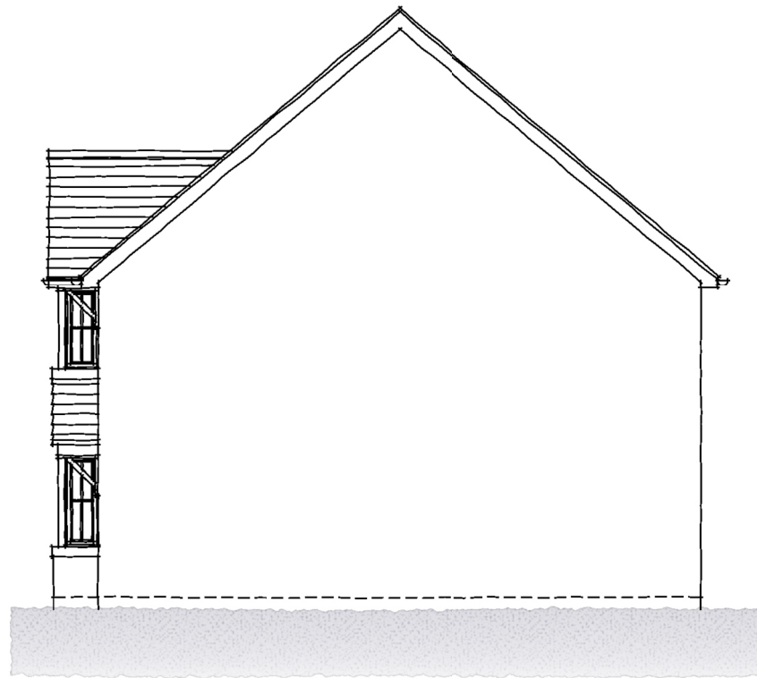
SIDE ELEVATION
