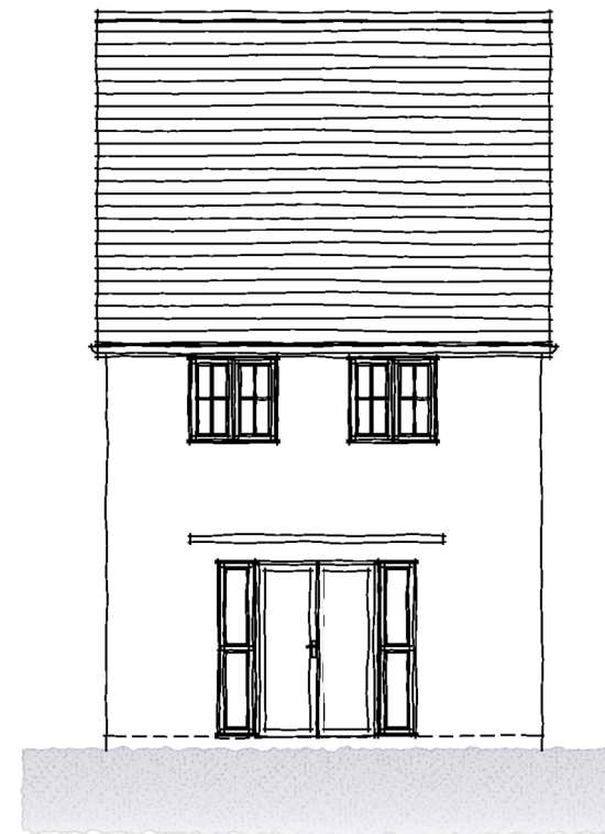
REAR ELEVATION
