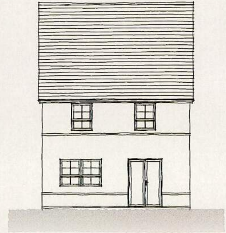
REAR ELEVATION
