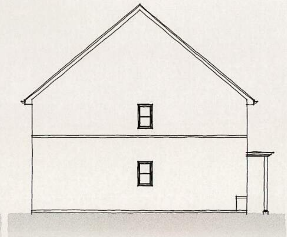
SIDE ELEVATION
