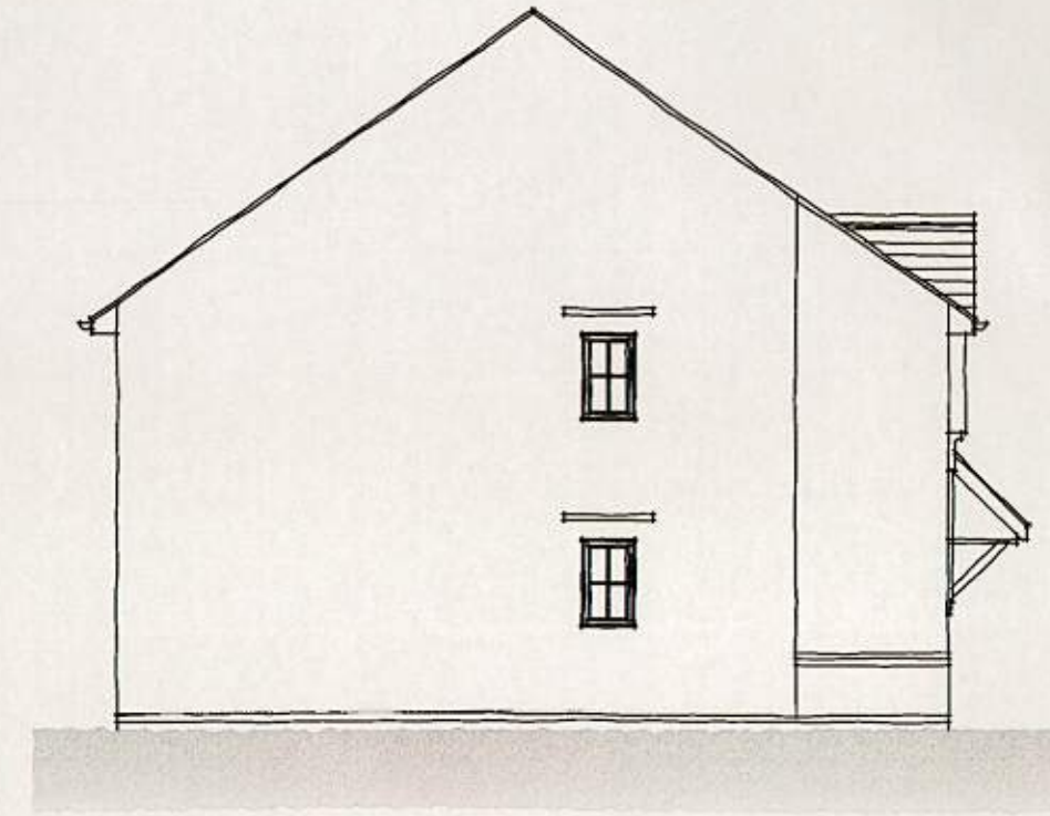
SIDE ELEVATION
