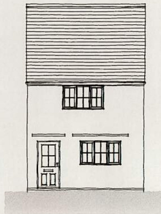
REAR ELEVATION
