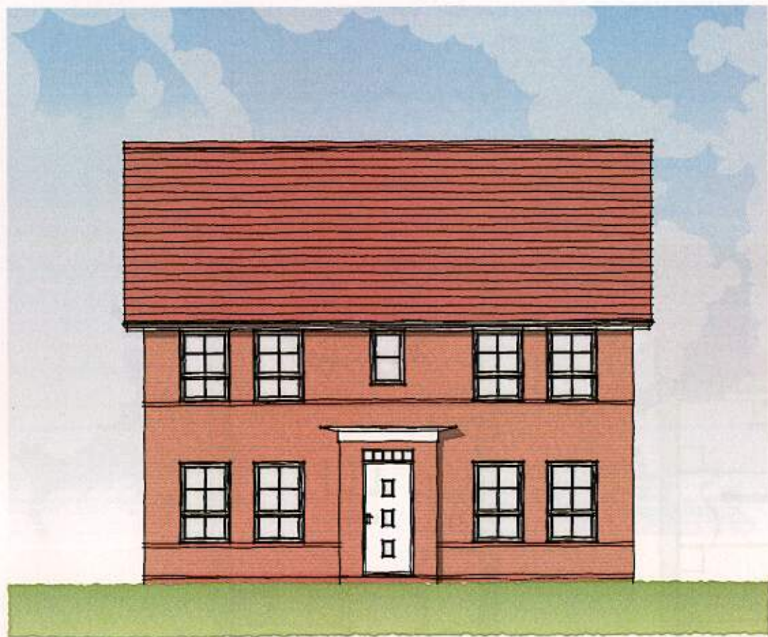
FRONT ELEVATION
