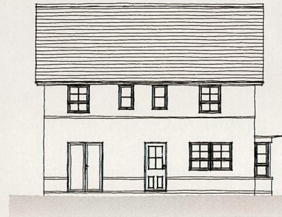
REAR ELEVATION
