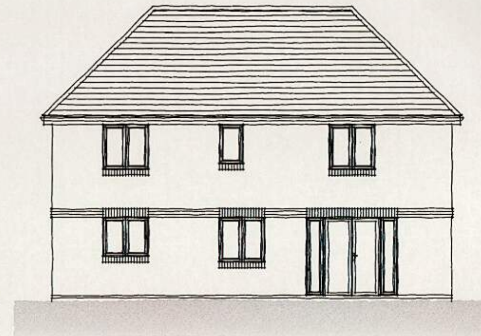
REAR ELEVATION
