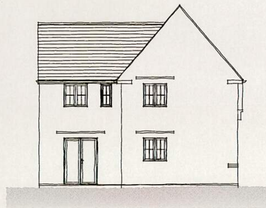
REAR ELEVATION
