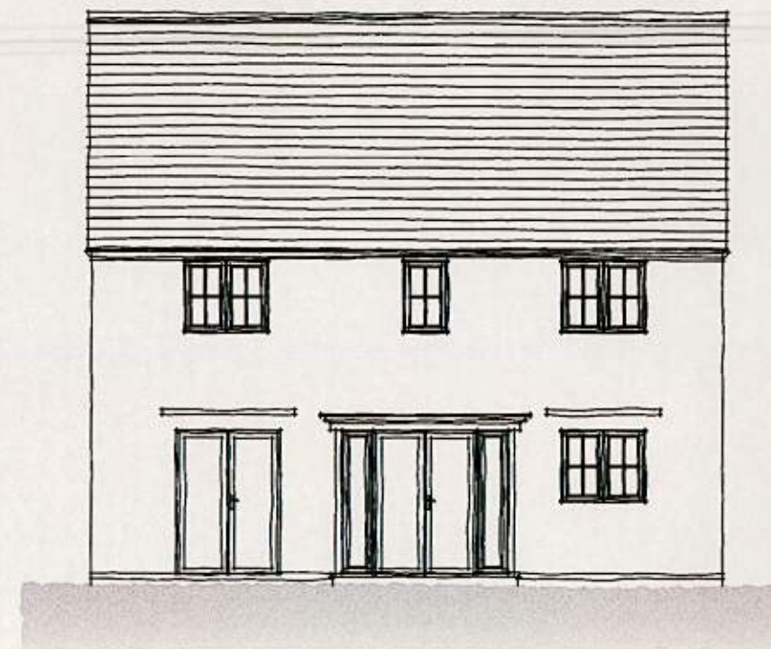
REAR ELEVATION
