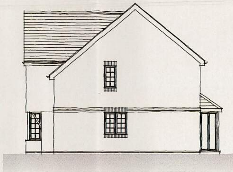
SIDE ELEVATION WINDOWS NOT TO PLOT 291
