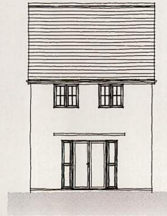
REAR ELEVATION
