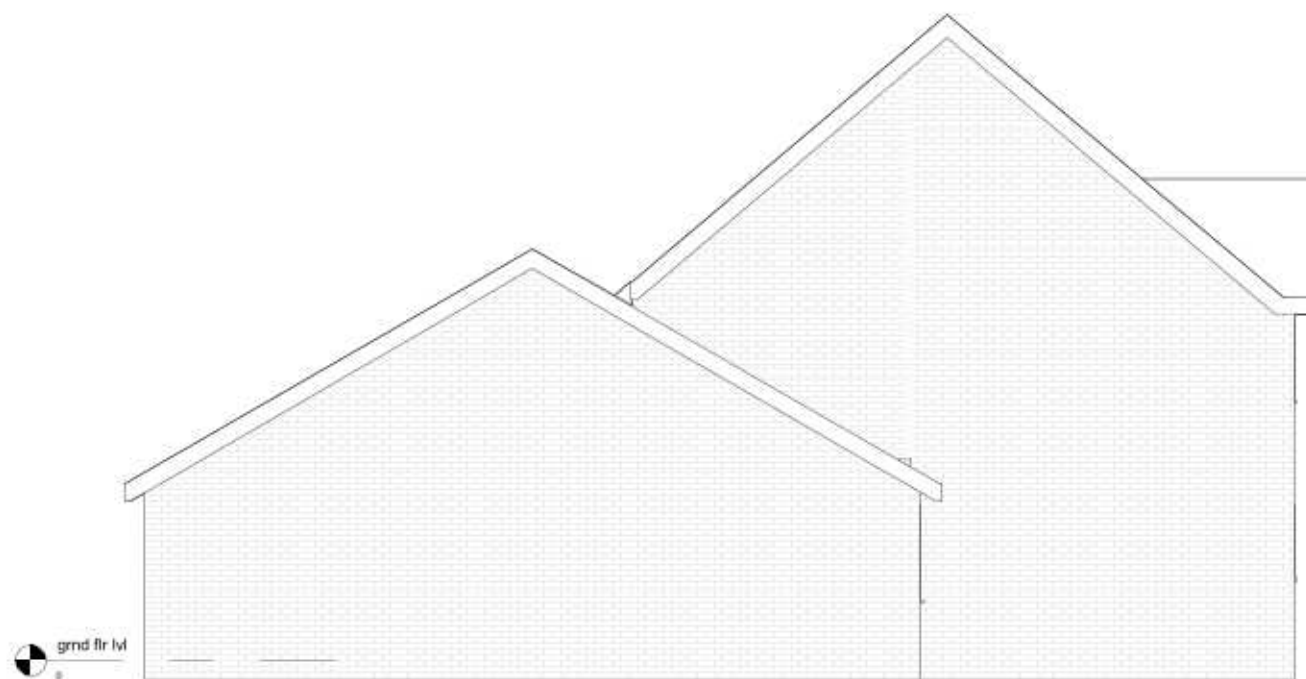
Existing Elevation-Left side
