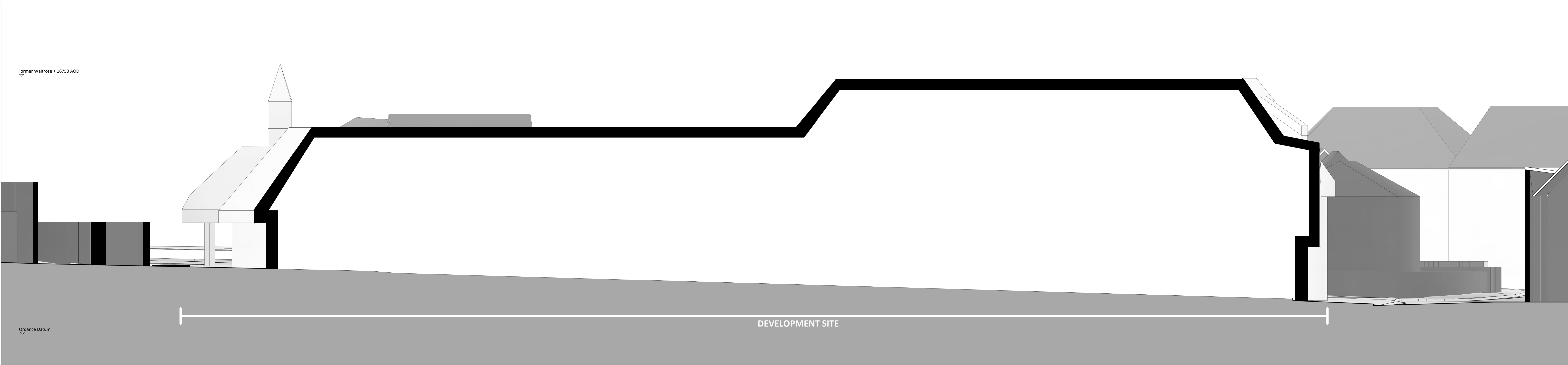
128_TPE_3030 | SECTION D-D | 1:100 @ A0
