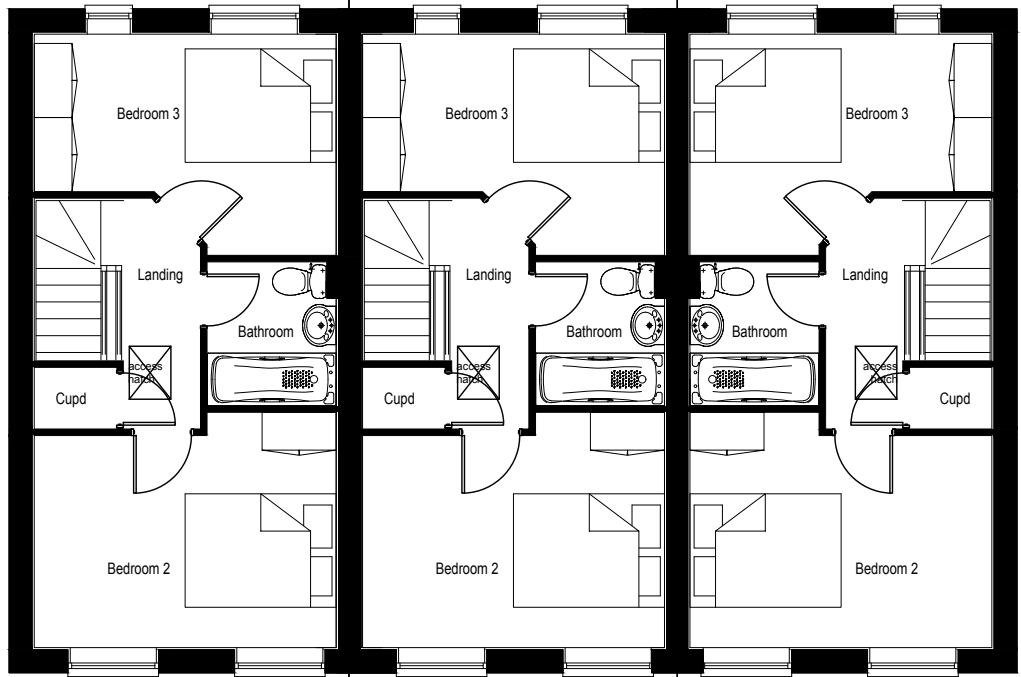
Second Floor Plot 49
