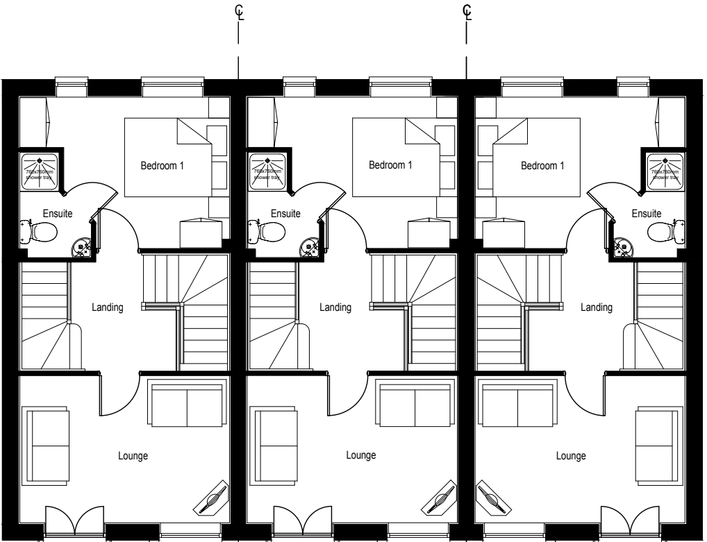
First Floor Plot 49
