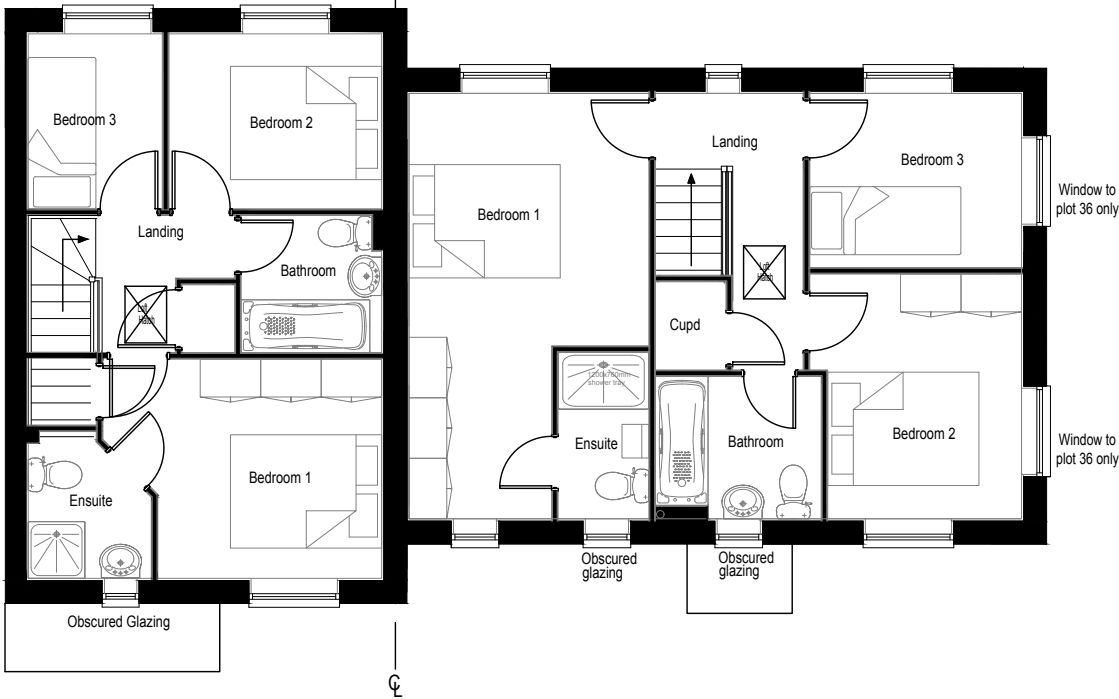
Hanbury - First Floor
