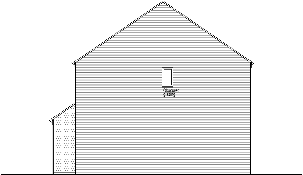
Side Elevation Plot 77
