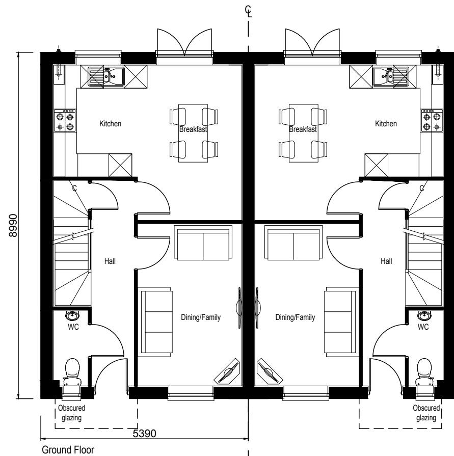
Ground Floor Plots: 41, 52, 102, 103
