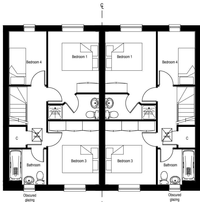
Second Floor Plots: 41, 52, 102, 103
