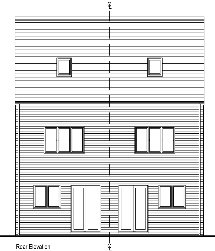
Rear Elevation Plots: 45, 48 Plots: 46, 47
