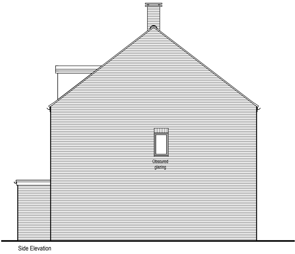
Side Elevation
