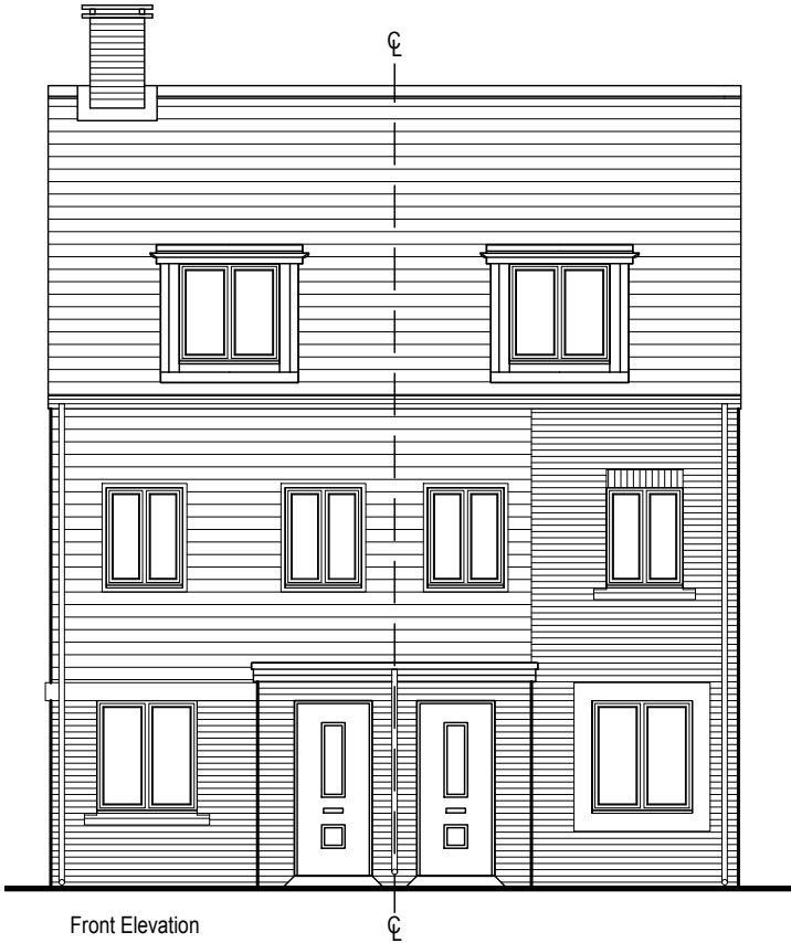
Front Elevation
