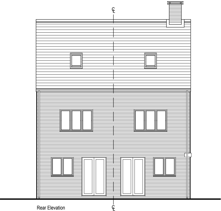
Rear Elevation
