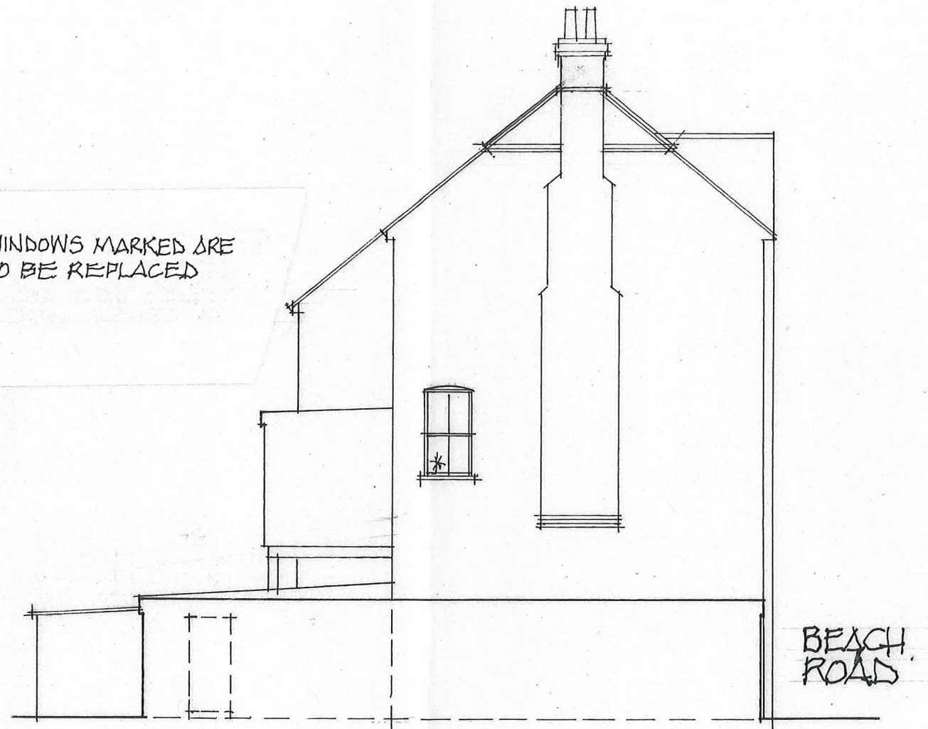
SOUTH ELEVATION - AS EXISTING
