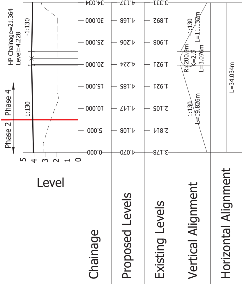
LONGITUDINAL SECTION ALONG ROAD 6
