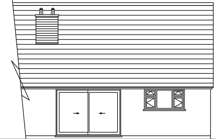
Existing West Elevation
