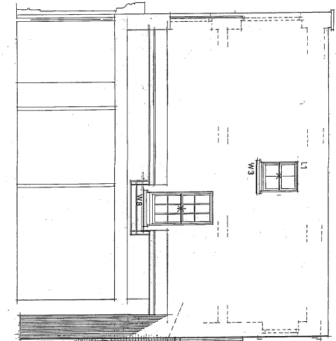
Section A-A / East Elevation
