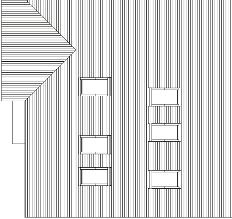
Proposed Roof Plan 1 : 100
