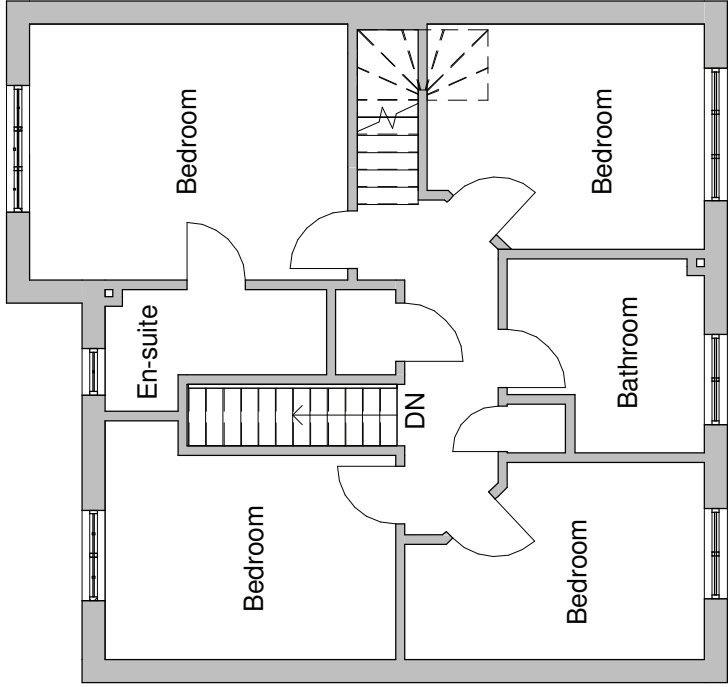
Proposed First Floor 1 : 100
