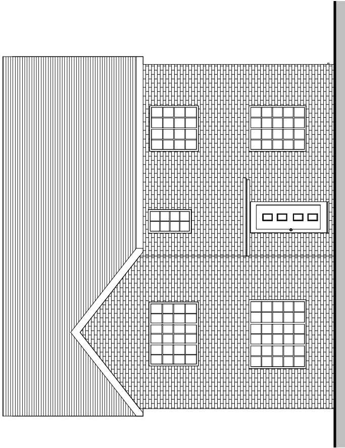
Existing NE Elevation
