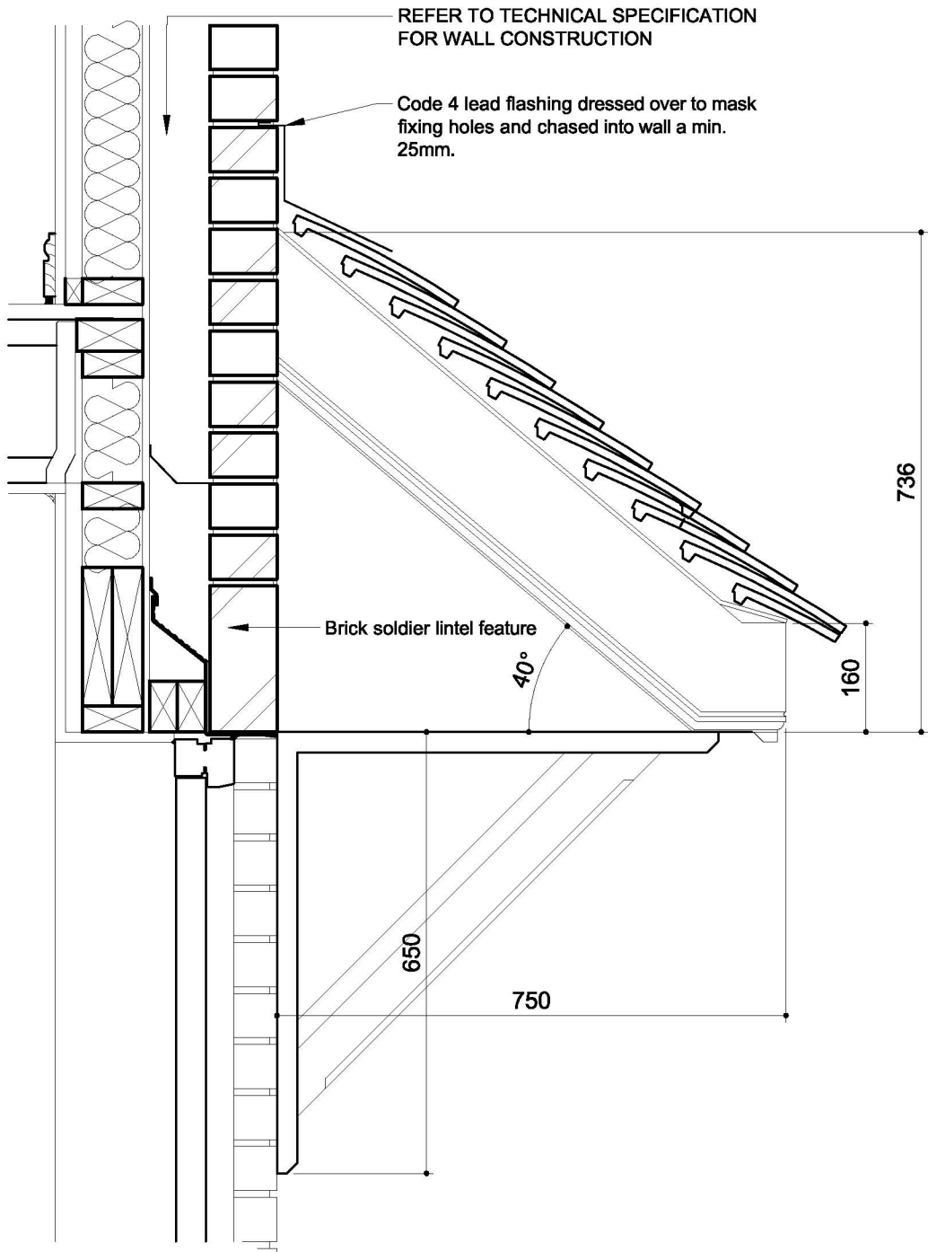
SIDE VIEW
