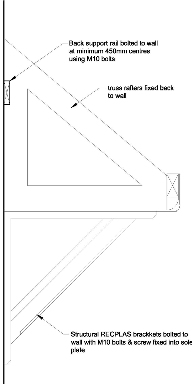
SECTION
