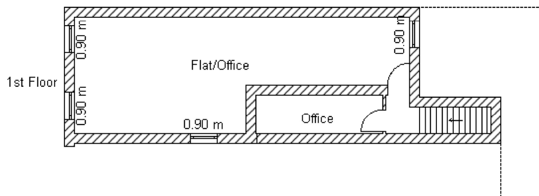
Proposed Floor Plans Scale 1:100
