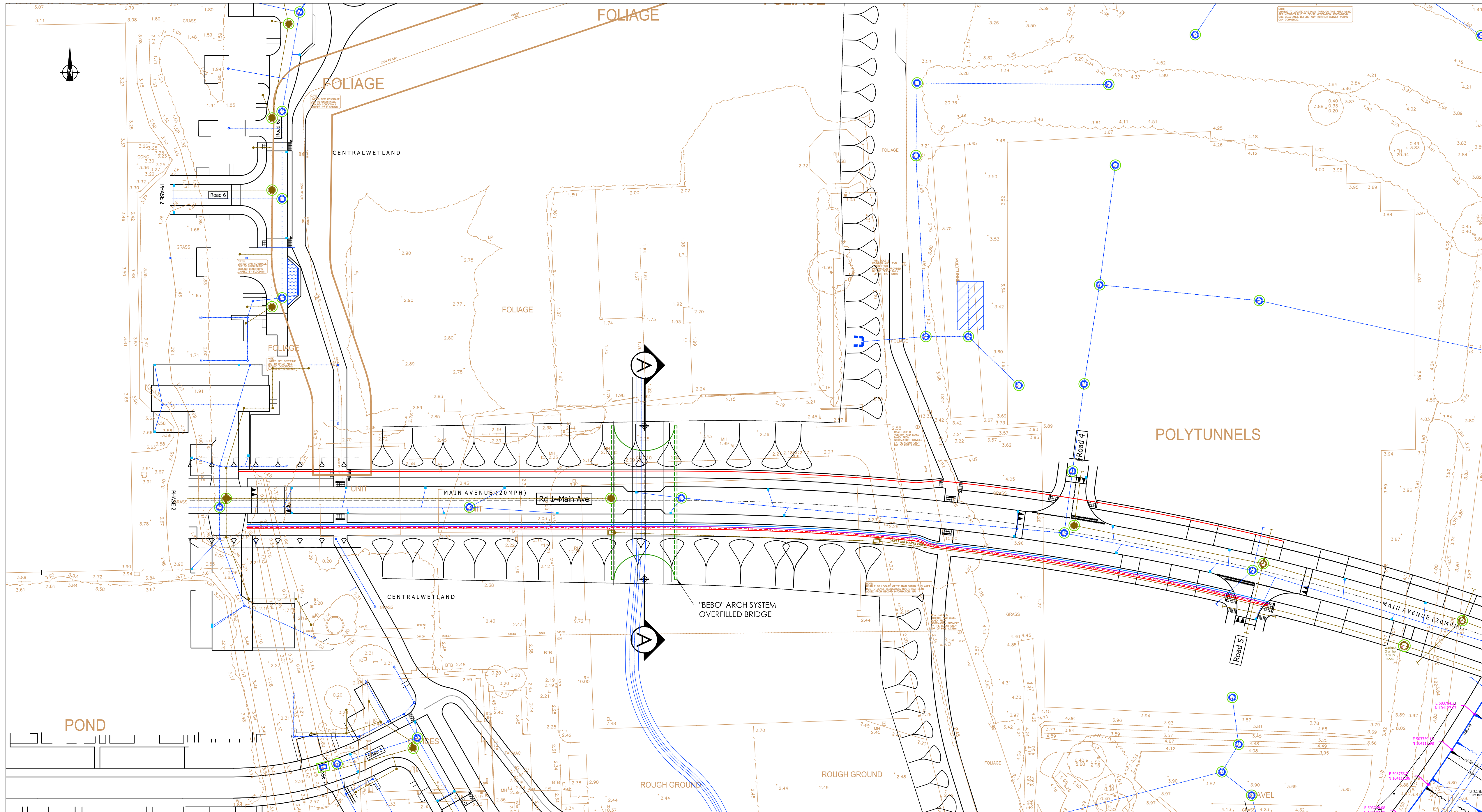
PLAN SCALE 1:500
