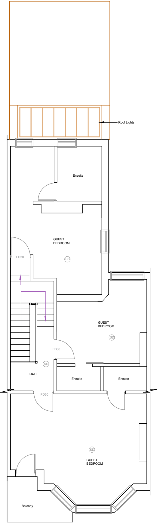
FIRST FLOOR
