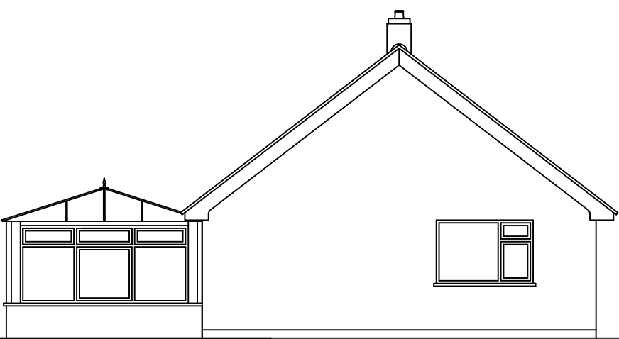
Existing Side/NW Elevation
